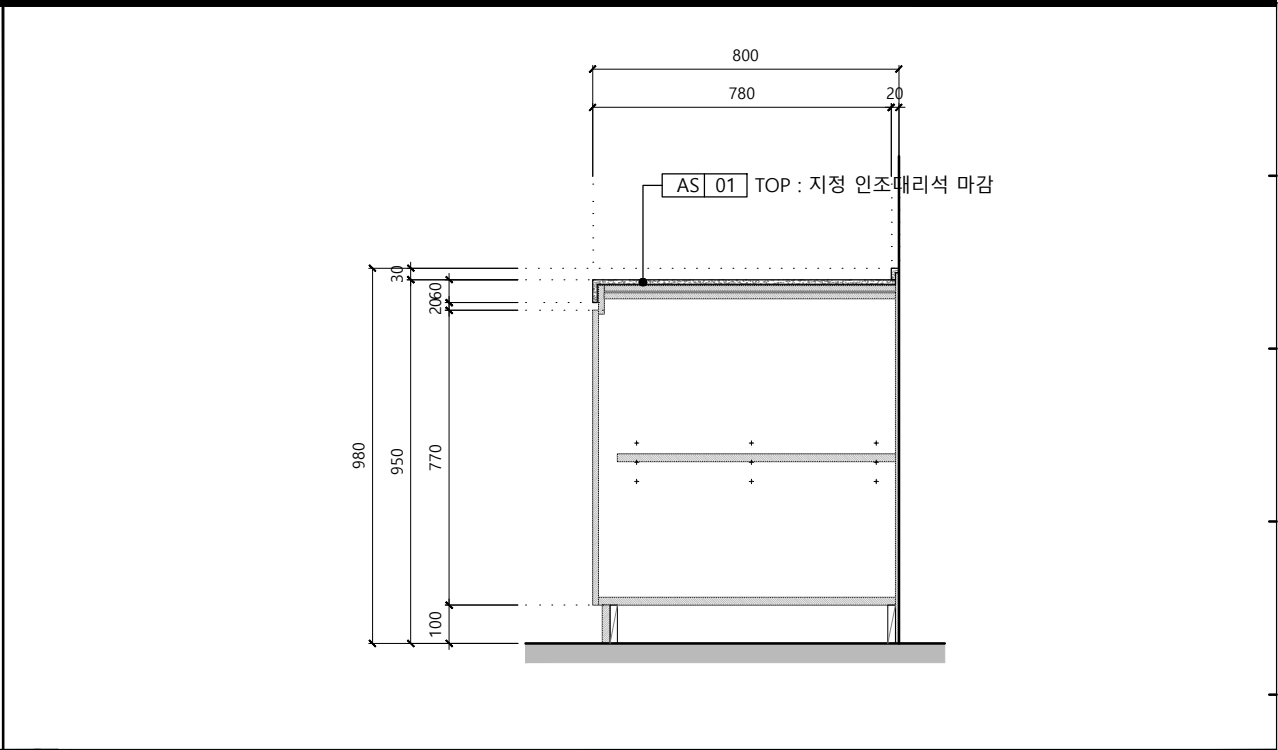
3 SIDE SECTION VIEW
