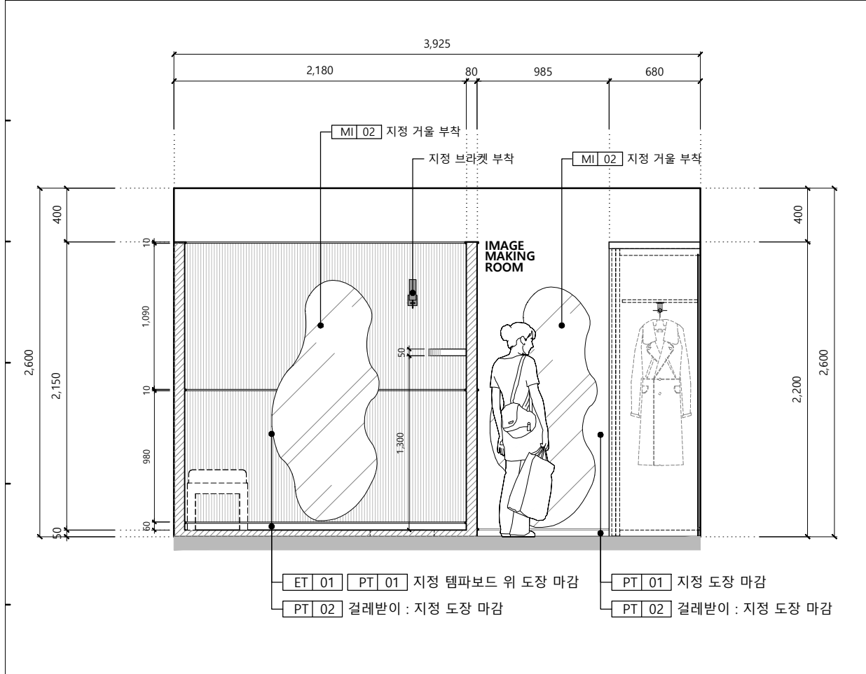
3 IMAGE MAKING ROOM _ ELEVATION
