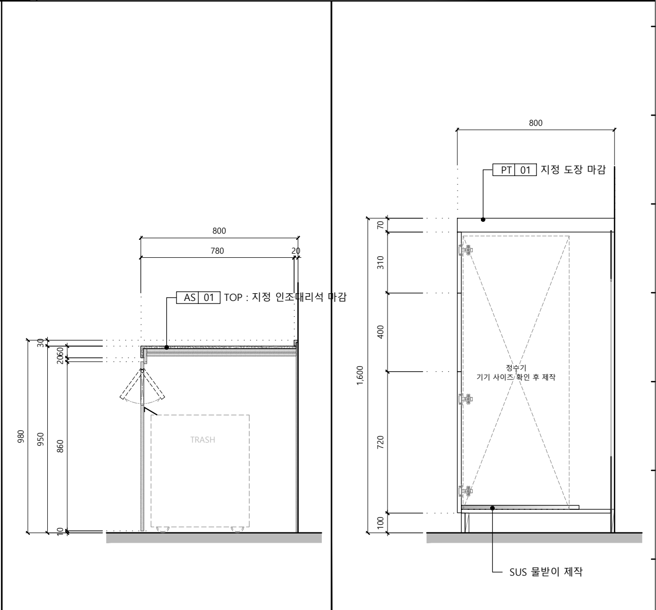
4 SIDE SECTION VIEW
