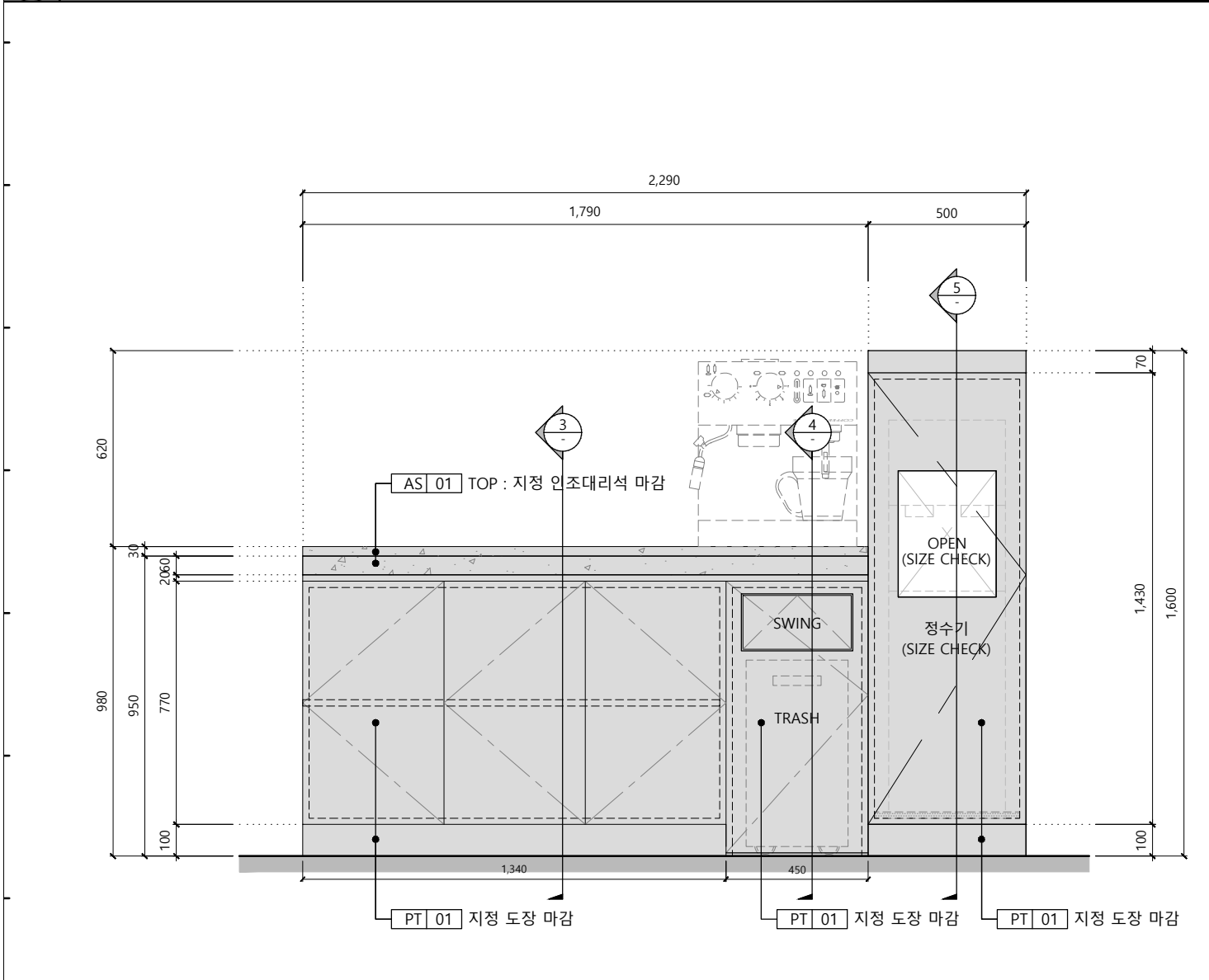
2 FRONT VIEW
