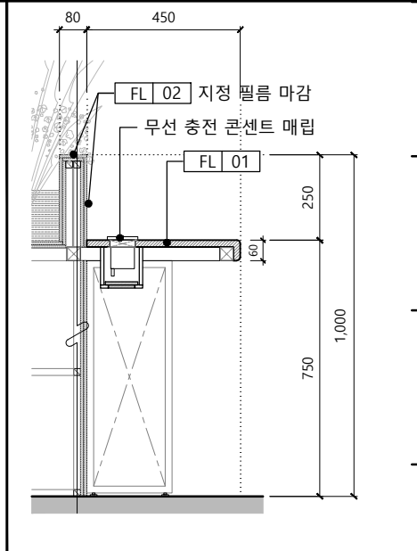
7 SECTION-3
