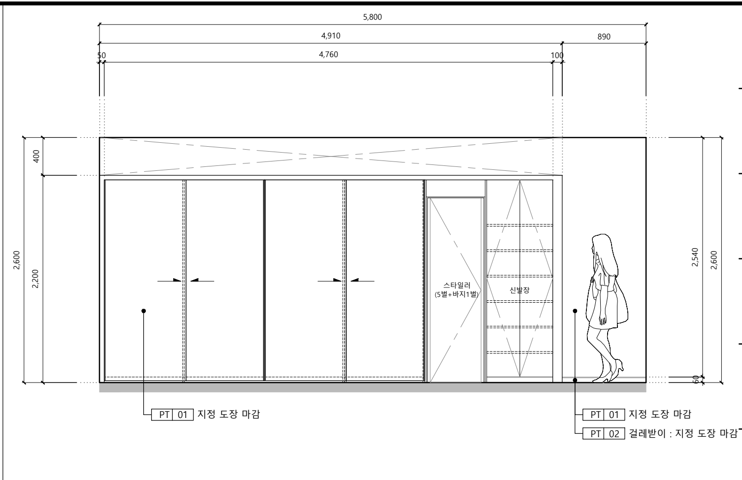
2 IMAGE MAKING ROOM _ ELEVATION
