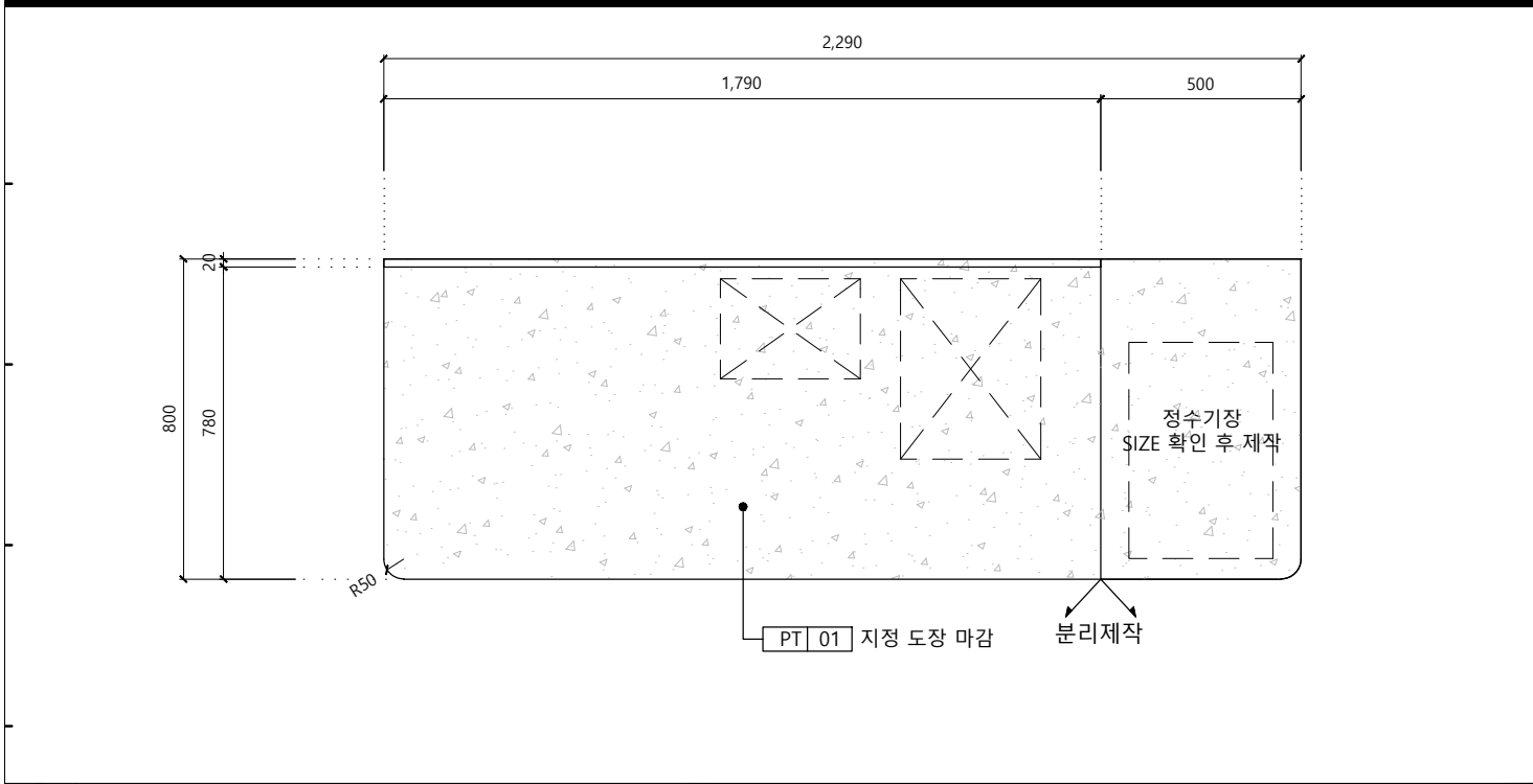
1 TOP VIEW
