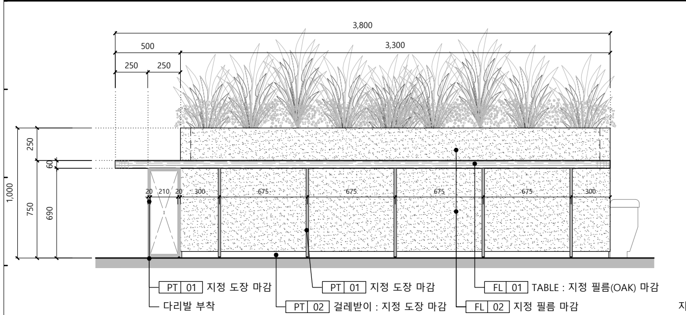
2 FRONT VIEW
