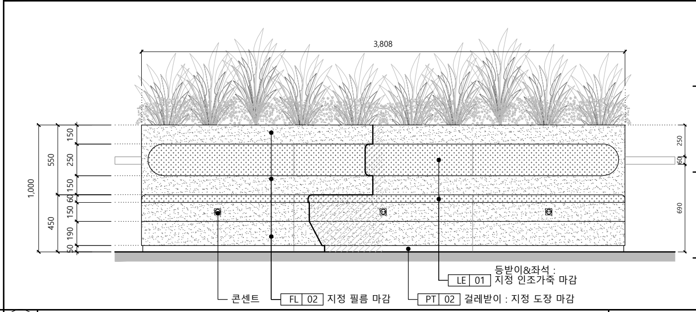
4 SIDE VIEW
