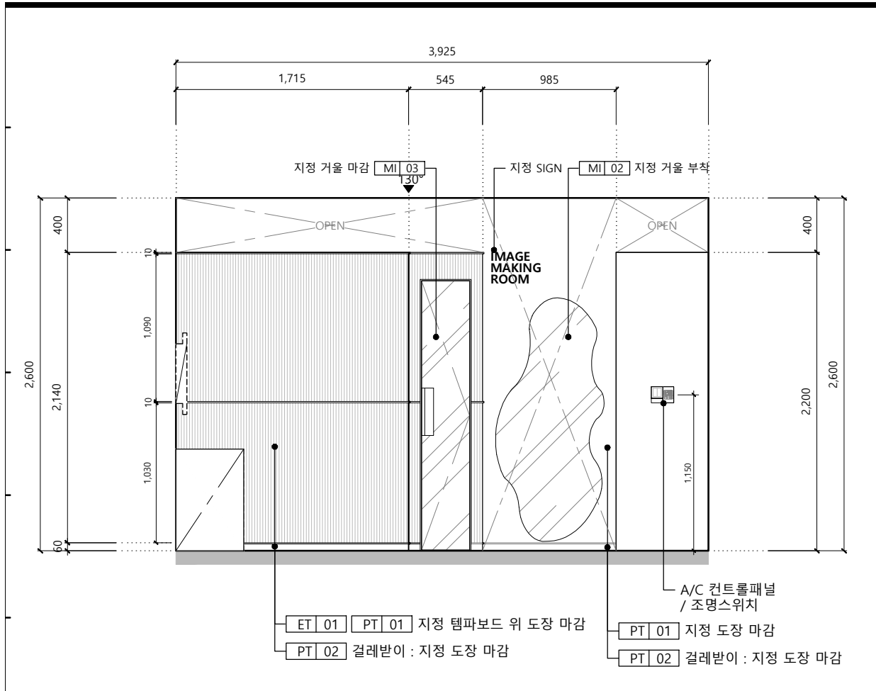
1 IMAGE MAKING ROOM _ ELEVATION
