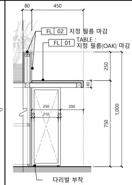
6 SECTION VIEW-2
