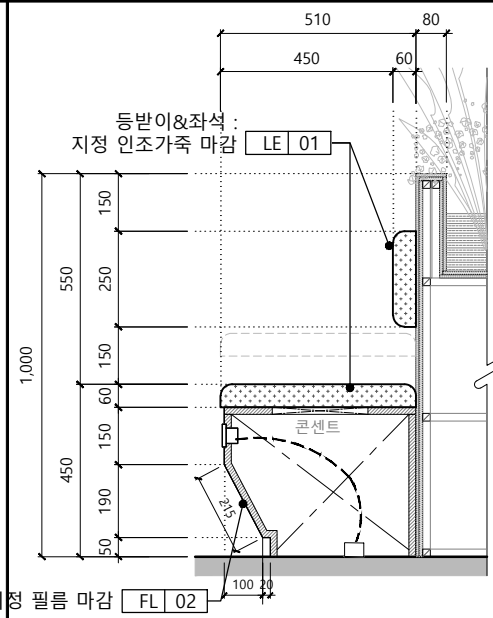
5 SECTION VIEW-1
