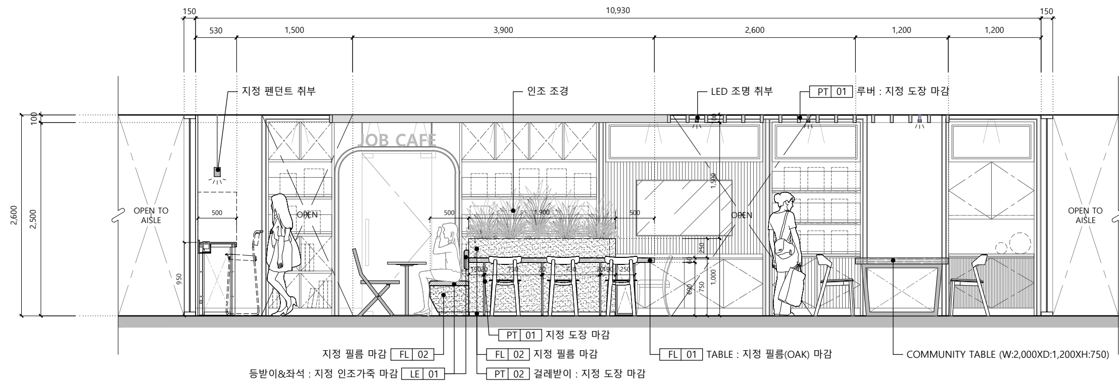
(2) JOB CAFE _ ELEVATION
